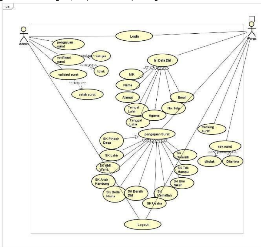
Gambar 2. Usecase Diagram
